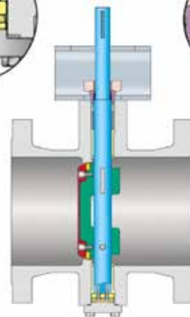
Double Shaft Blowout Protection
